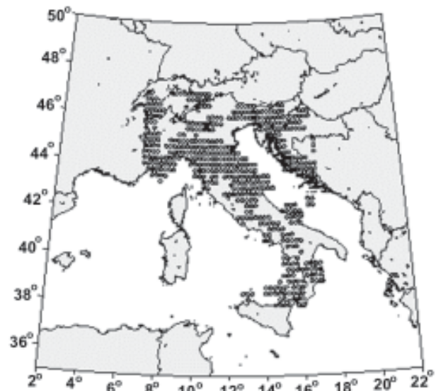
Figure 1. The territory singled out by the procedure, as on 2001.01.01, for the prediction of earthquakes with magnitude 6.5 and above. Each dot corresponds to the center of a circle of investigation to which the M8 algorithm is applied.
