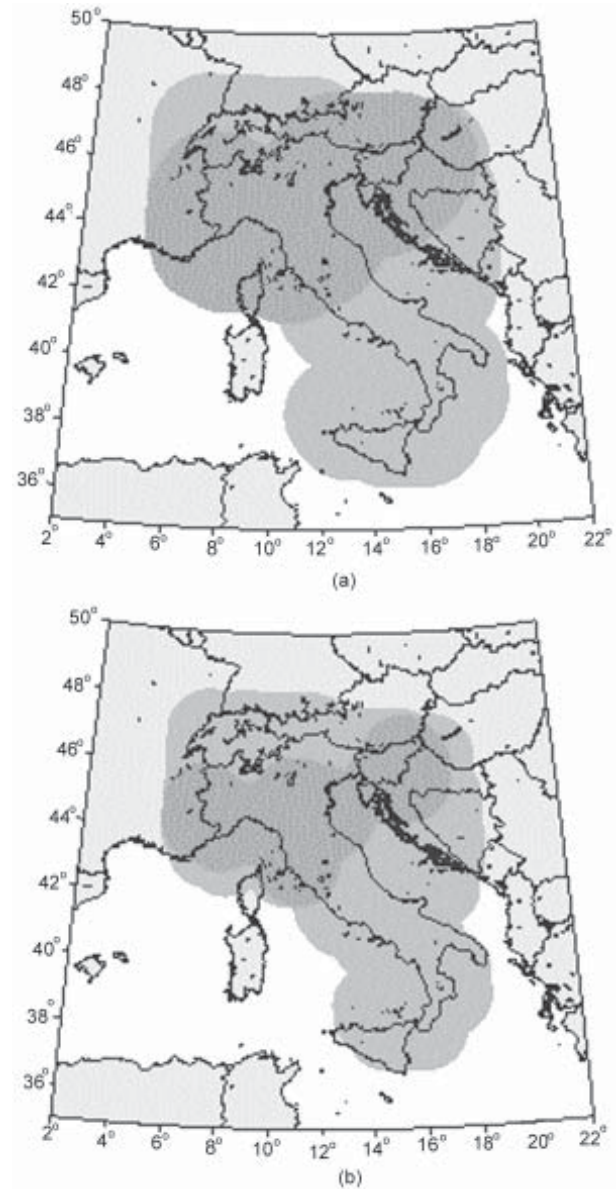
Figure 3. The current alarms determined with algorithm M8 in Italy, as on 2001.07.01 (subject to update in January 2002), for (a) M_0=6.5 and (b) M_0=6.0 .
