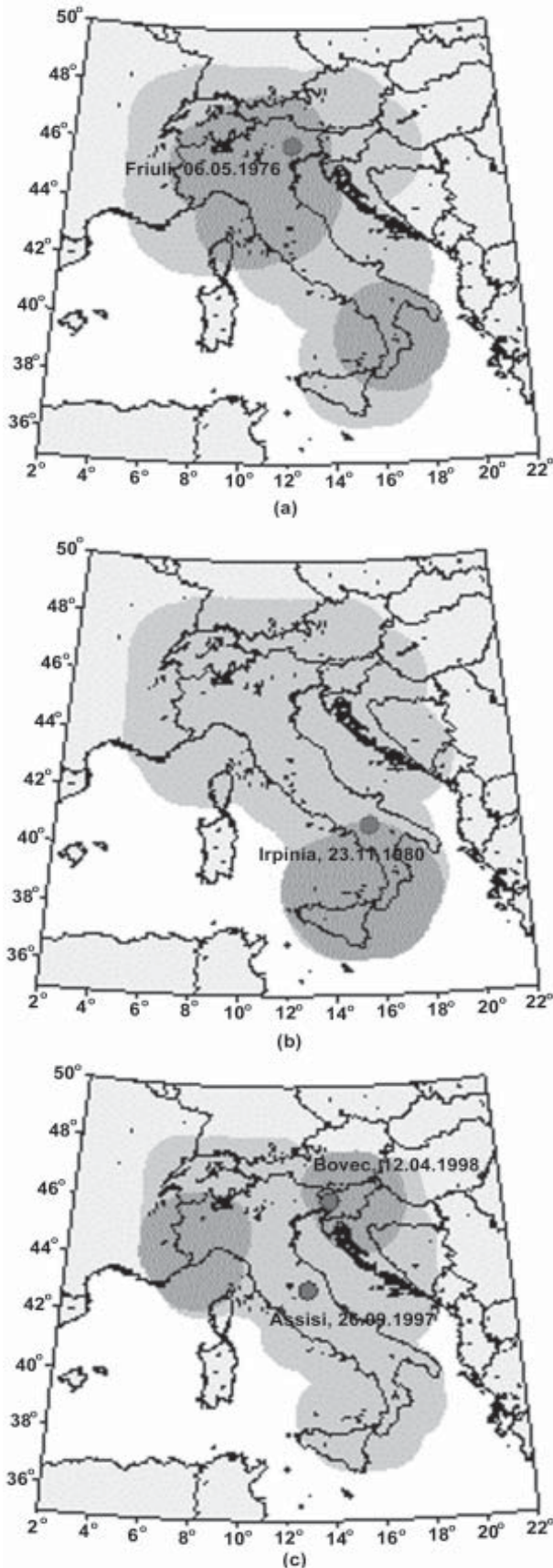
Figure 2. Results of the prediction obtained with the new space stabilized variant of algorithm M8. Application in Italy for M_0=6.5 before (a) the Friuli 1976, M_{max}=6.5 and (b) the Irpinia 1980, M_{max}=6.7 earthquakes. (c) Same for M_0=6.0 before the Bovec 1998, M_{max}=6.0 earthquake, M_{max} is the largest value of the magnitudes reported for each event.
