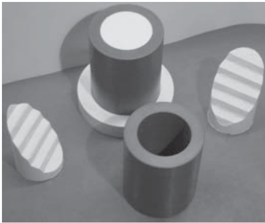
a) Triaxial samples.
