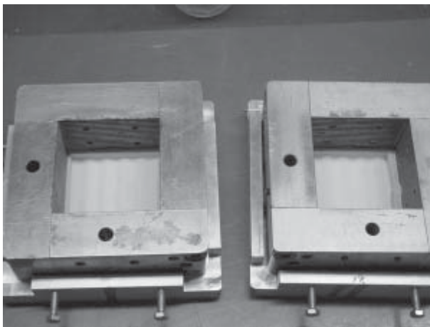
b) Direct shear samples.
