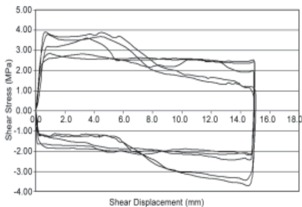
Figure 16. Shear stress-shear displacement curve for saw-tooth sample during 5 cycles in 4.2 MPa normal stress.
