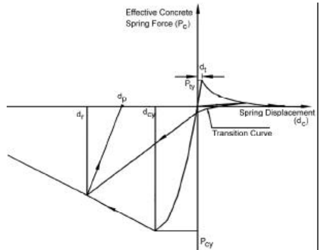
Figure 5. Hysteretic response for concrete spring [18].
