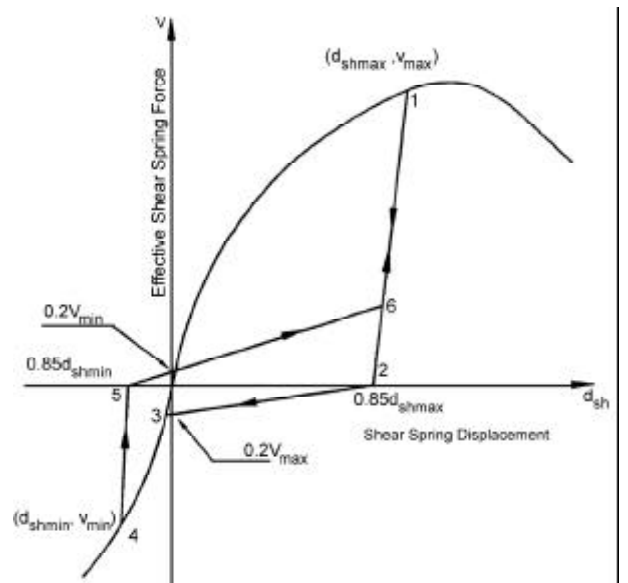
Figure 6. Hysteretic response for shear spring [18].
