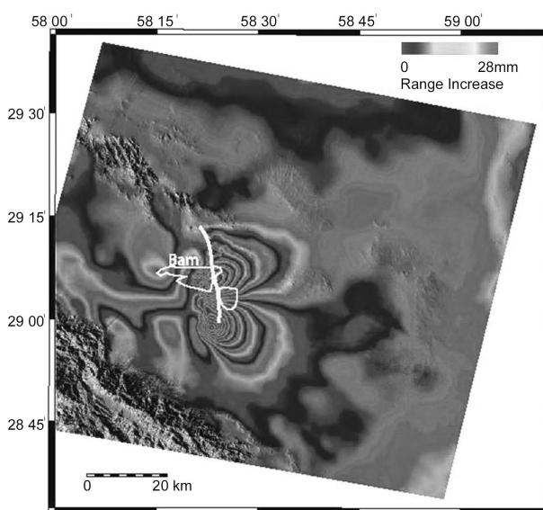
Figure 3. Co-seismic differential ASAR Interferogram in descending orbits [03 Dec 03 - 07 Jan 04], using SRTM dem. The altitude of ambiguity is 20m.
