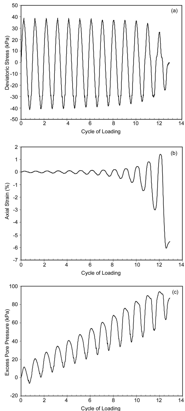
Figure 2. Typical cyclic triaxial test data, fines content=50%, \sigma'_C = 100\text{kPa} . (a) deviatoric stress vs number of cycles, (b) axial strain vs number of cycles, (c) excess pore pressure vs number of cycles.
