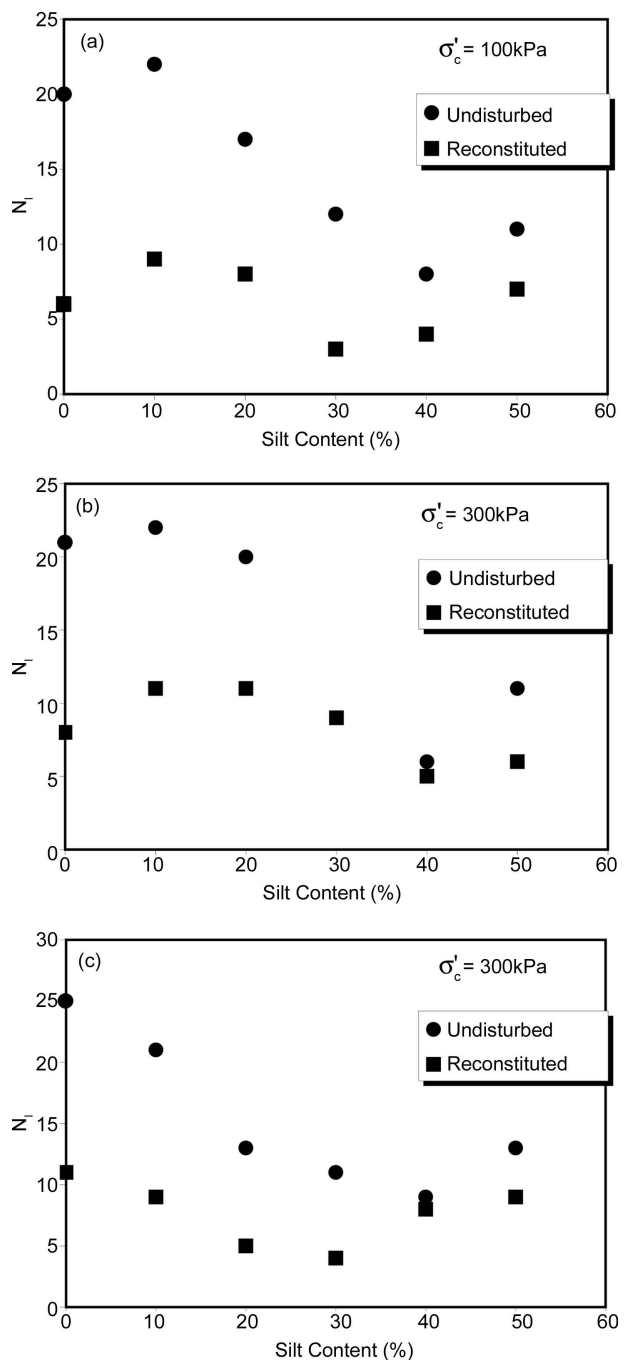
Figure 3. Variation in N_l with silt content for undisturbed and reconstituted specimens.
