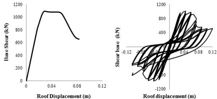
Figure 8. Structural behavior of Khurjini frame under cyclic load and pushover result
