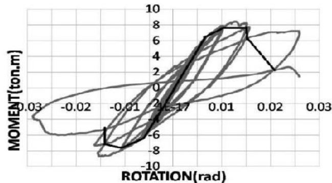
Figure 4. Moment-rotation curve of Khorjini connections utilized in this study Amiri and Aghakhouchak (2011)
