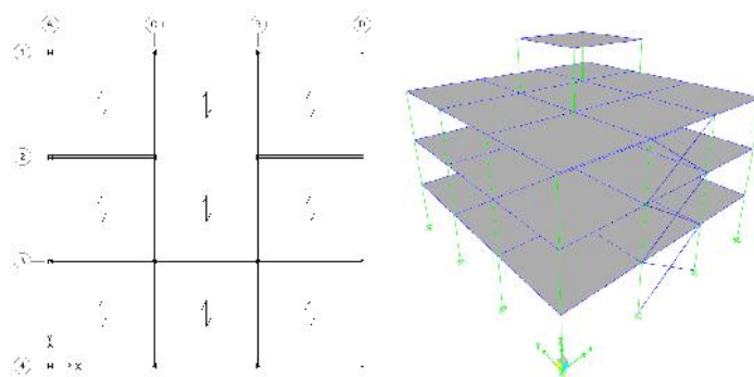
Figure 2. Plan view and 3D view of 3-story conventional building models
