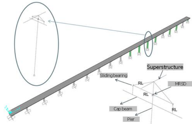
Figure 8. Structural model of the bridge
