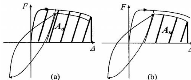
Figure 11. Definition of damage equation parameters of the model by Hindi and Sexsmith (2001):(a) monotonic energy in the virgin state; (b) monotonic energy after the application of load-displacement cycles
