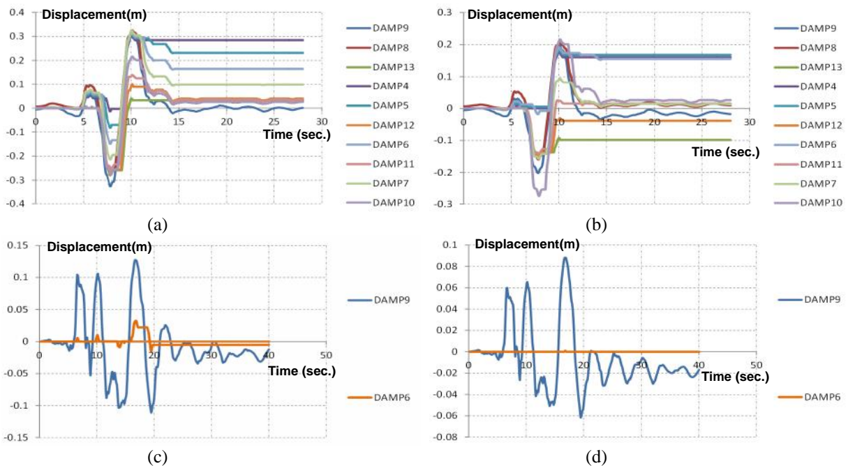
Figure 9. Displacement response history of dampers in the longitudinal direction for (a) Kocaeli, MCE; (b) Kocaeli, DBE; (c) Landers, MCE and (d) Landers, DBE earthquake records
