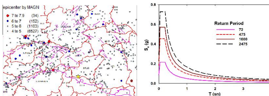
Figure 3. (a) Site seismicity (the site is shown by a yellow star); (b) Site-specific design spectrum
