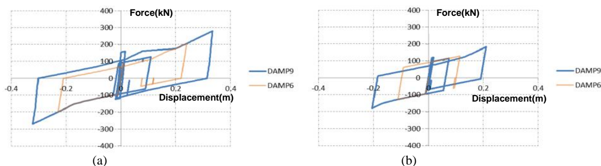
Figure 9. Sample hysteresis loops of damper on piers No. 6 and 9 in the longitudinal direction for (a) Kocaeli, MCE and (b) Kocaeli, DBE earthquake records
