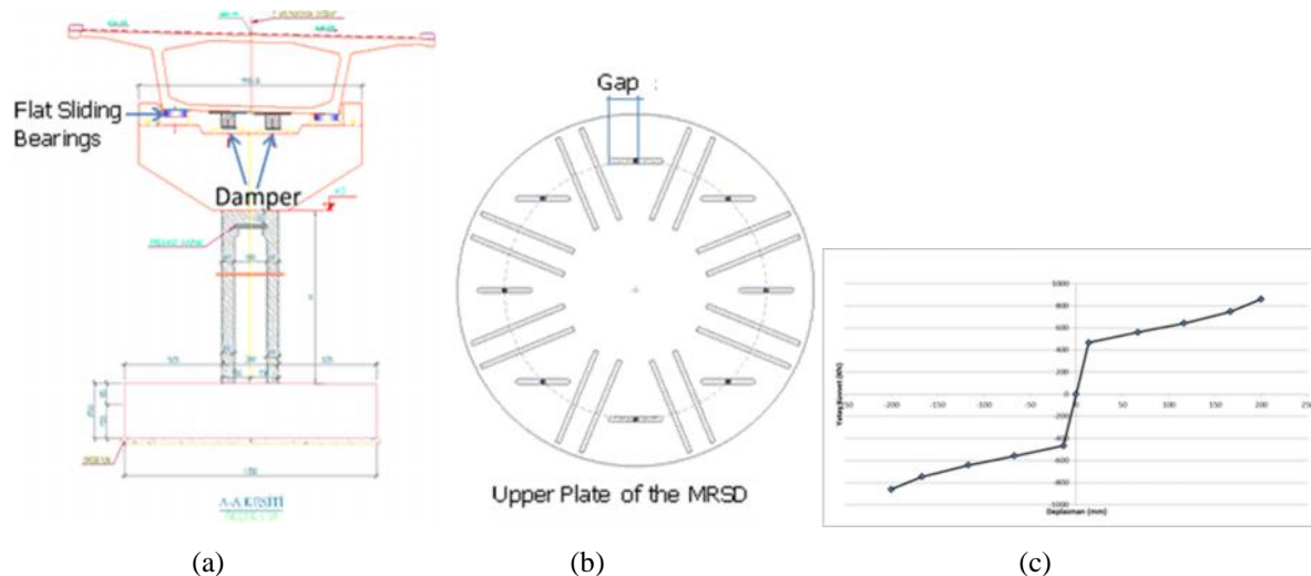
Figure 7. (a) Installation of two MRSDs on a typical pier; (b) The provided gaps (logitudinal direction) on the upper plate of the MRSDs where the device is mounted to the deck; (c) Force-displacement response of MRSD
