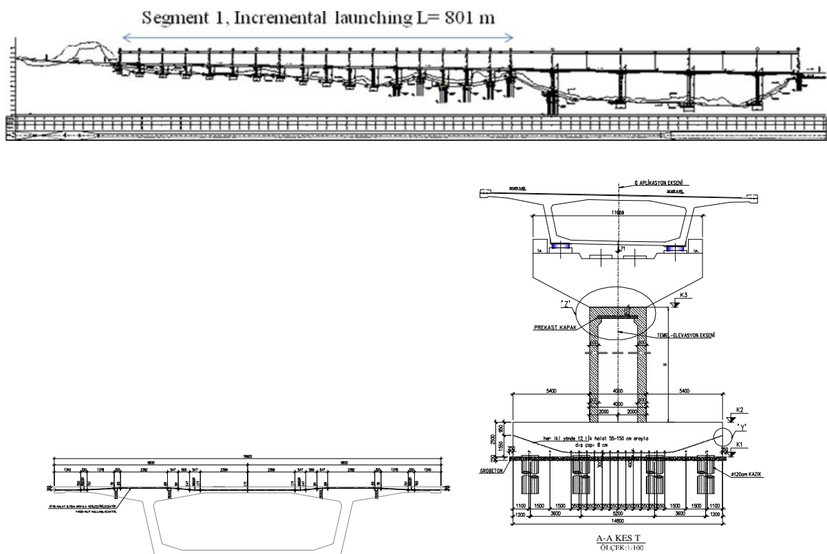
Figure 2. Longitudinal and cross-section views of the bridge and the deck
