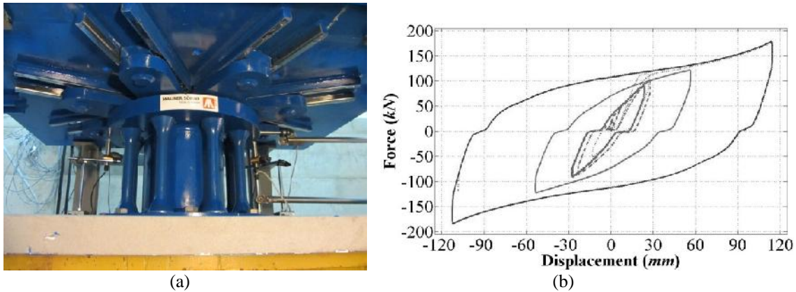
Figure 5. (a) 200kN, 120mm-capacity prototype MRSD; (b) Cyclic response obtained from tests
