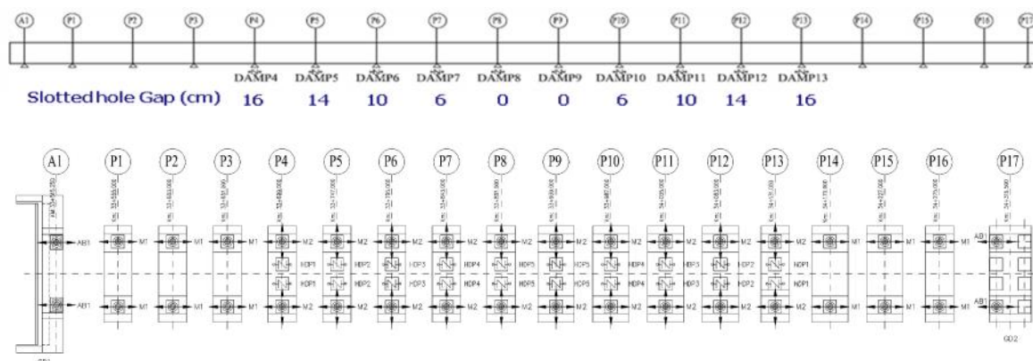
Figure 6. Schematics of the isolation system
